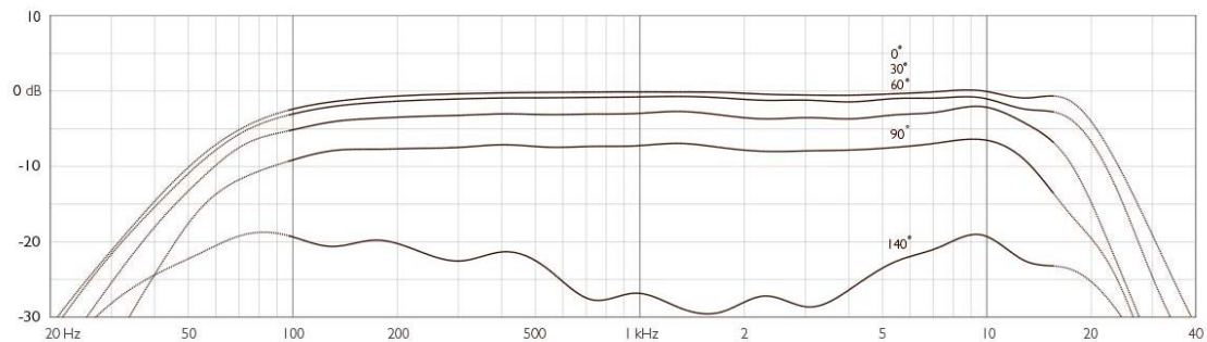
Typical on and off-axis response of a d:facto™ 4018VL
