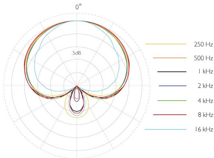
Typical directional characteristics of a d:facto™ 4018VL
